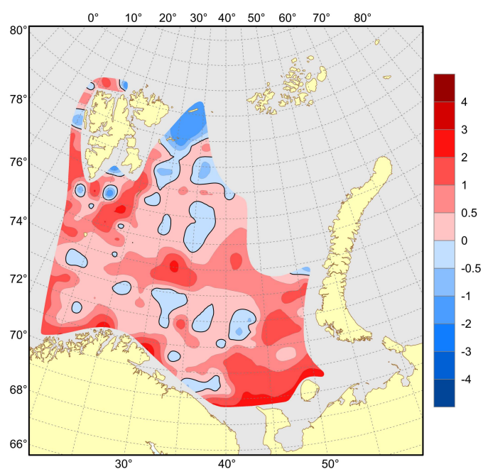
Figure 4.1.1.10. Bottom temperature anomalies ( ^{\circ}\text{C} ), August–November 2022.
