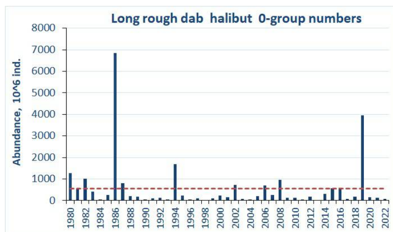
Figure 6.9.2. 0-group long rough dab abundance estimates were not corrected for capture efficiency for the period 1980-2022. Red line shows the long-term average.
