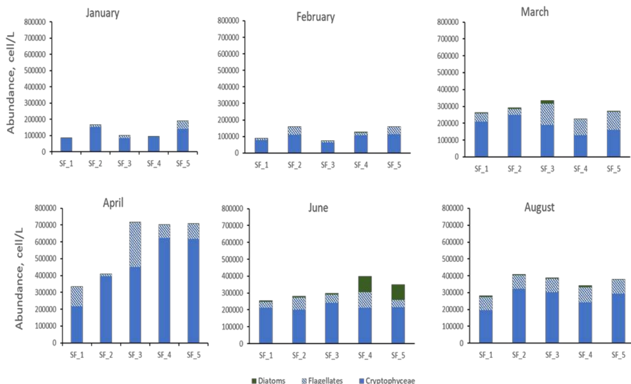
Figure 4 Phytoplankton abundance presented for all months and station. In blue phytoplankton cells smaller than 5 \mu m while in green is the diatom contribution.
